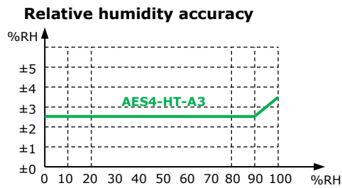
Figure 1: Max RH-tolerance at 25 °C (77 °F)
