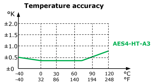
Figure 2: Max Temperature-tolerance
